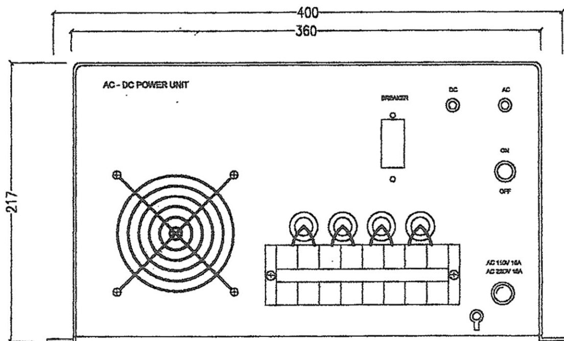
FRONT VIEW SCALE 1 : 3
